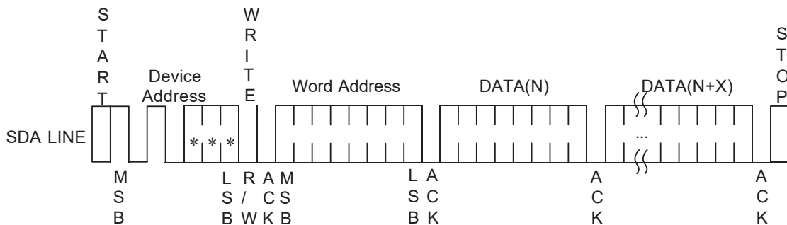
Figure 4: Page Write
