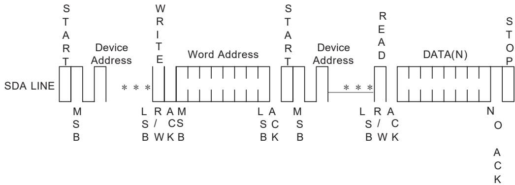
Figure 7: Random Read
