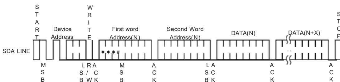
Figure 4: Page Write
